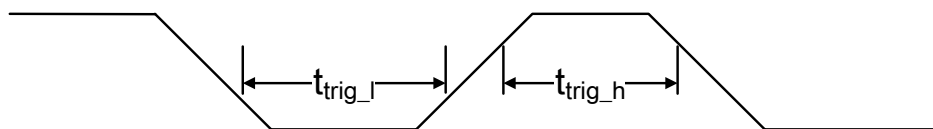
Figure 2-7 Hardware trigger timing
